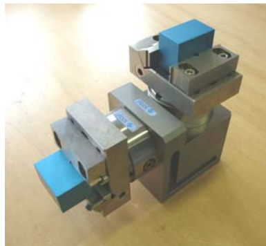
Example of a Multi vise setup
